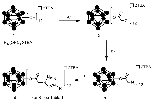
Scheme 1. Synthetic route for twelve-fold click reaction with [\text{closo-B}_{12}(\text{OH})_{12}]^{2-} . Conditions: a) chloroacetic anhydride in \text{CH}_3\text{CN} , 5 d, reflux; b) \text{NaN}_3 in DMF, 2 d, 50 °C; c) alkyne, CuI, DIPEA, \text{CH}_3\text{CN}/\text{THF} (1:1), 2–3 d, RT. DIPEA = diisopropylethylamine.
